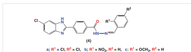
Figure 5 Cytotoxic compounds 4a-c
