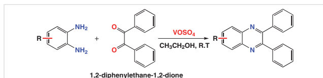
Scheme 10 Reaction of 1,2-diphenylethane-1,2-dione with o -phenylenediamine using VOSO 4 as catalyst
