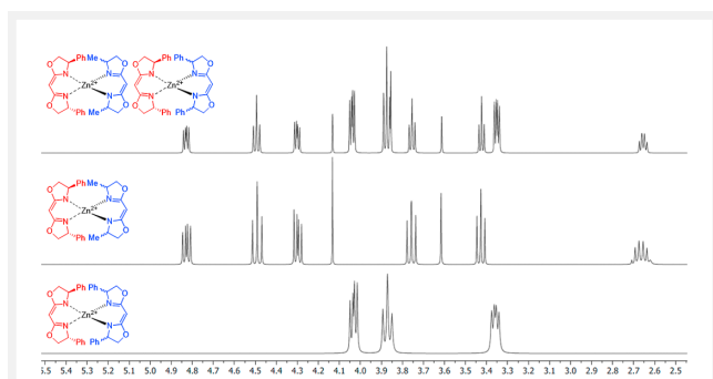
Figure 4 Comparison of ^1\text{H} NMR spectra: (SS,RR) -Zn(II) BOX (Ph/Ph) (bottom), (SS,RR) -Zn(II) BOX (Me/Ph) (middle), and formation of two specific heterochiral Zn(II) BOX complexes (top).
