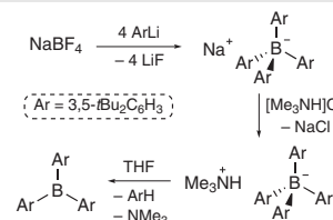
Scheme 1 Synthesis of B(3,5- t Bu 2 C 6 H 3 ) 3
