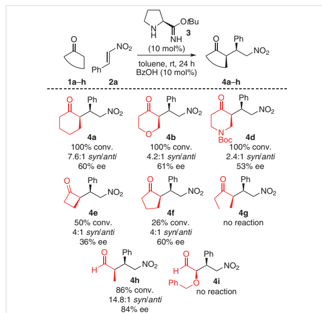
Scheme 3 Ketone and aldehyde scope with benzoic acid as an additive. The conversion and syn/anti ratios were determined by 400 MHz ^1\text{H} NMR spectroscopy after 24 hours. The ee was determined by chiral-stationary-phase HPLC (see Supporting Information).
