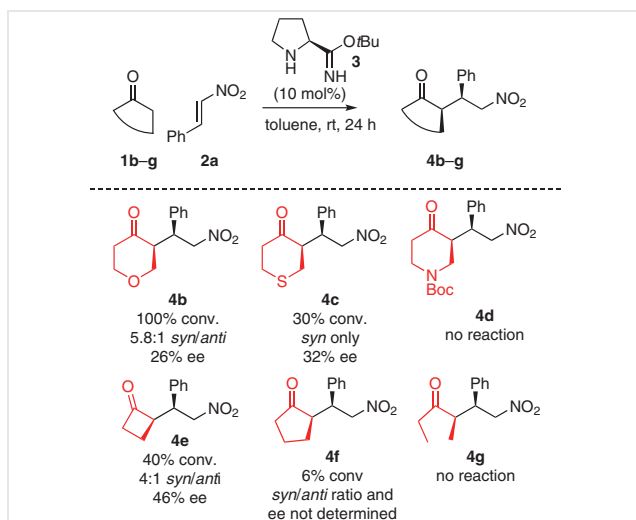
Scheme 2 Ketone scope. The conversion and syn/anti ratios were determined by 400 MHz ^1\text{H} NMR after 24 hours. The ee was determined by chiral-stationary-phase HPLC (see Supporting Information).
