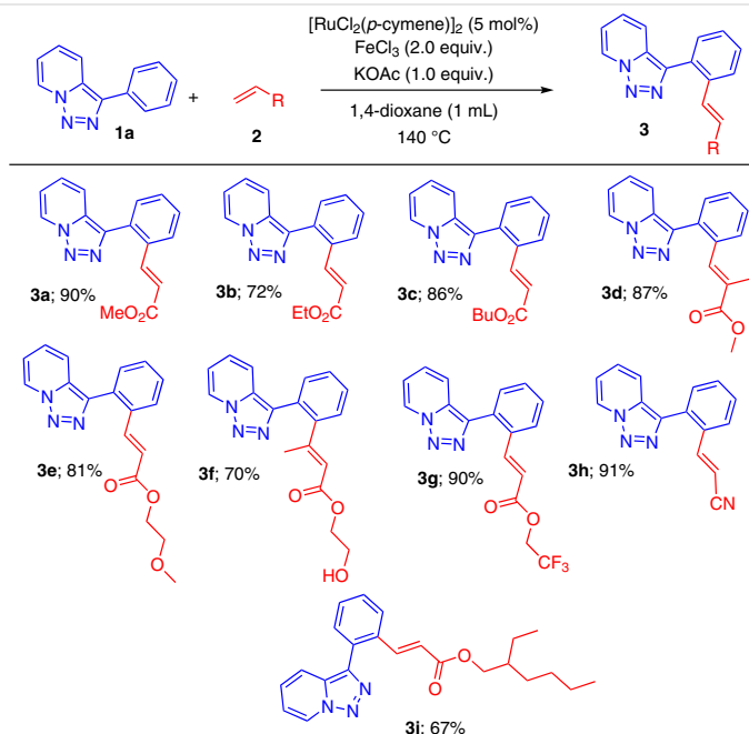
Scheme 2 Substrate scope of triazolo[1,5-a]pyridines. Reagents and conditions: 1a (0.25 mmol), 2 (0.5 mmol), catalyst (5 mol%), additive (2.0 equiv.), base (1.0 equiv.), solvent (1 mL), in an oil bath, isolated yield.
