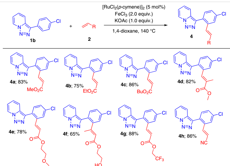
Scheme 3 Substrate scope with 3-(4-chlorophenyl)-[1,2,3]triazolo[1,5-a]pyridine. Reagents and conditions: 1b (0.25 mmol), 2 (0.5 mmol), catalyst (5 mol%), additive (2.0 equiv.), base (1.0 equiv.), solvent (1 mL), in carousel reaction station, 48 h, isolated yield.
