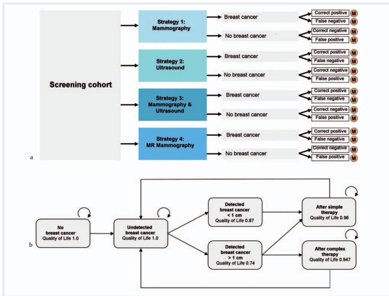
► Fig. 3 Illustration of a diagnostic decision model. a Decision model for screening patients for the presence of breast cancer. b Markov model for estimating long-term costs and long-term effectiveness.
