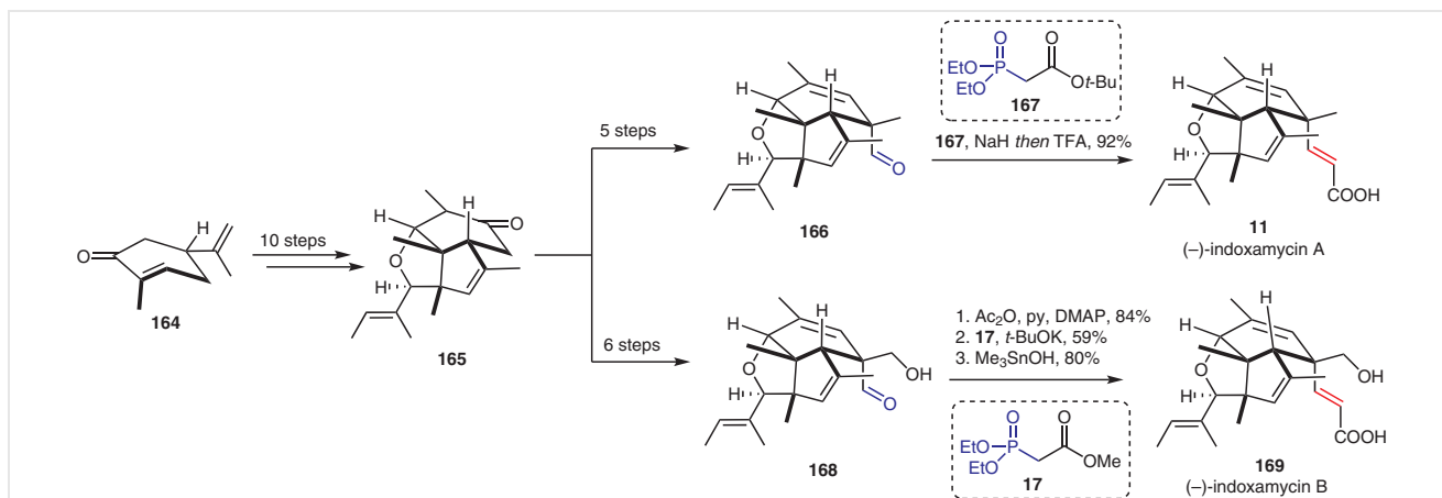
Scheme 17 Total synthesis of (–)-indoxamycins A and B by Liang and co-workers
