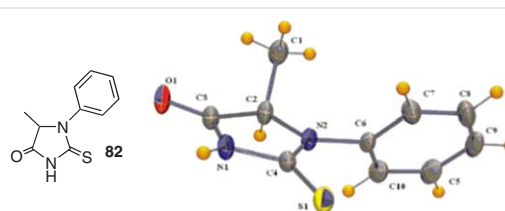
Figure 8 Crystal structure of 82 . (Reprinted with permission from ref. 95. © 2012 Elsevier Ltd.)
