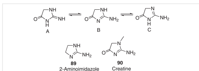
Figure 9 Tautomeric forms of 2-imino-hydantoin
