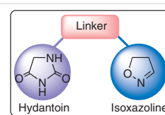
Figure 11 Molecular design of hydantoin–isoxazoline hybrids
