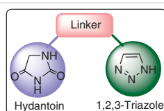
Figure 10 Molecular design of novel hydantoin–1,2,3-triazole hybrids
