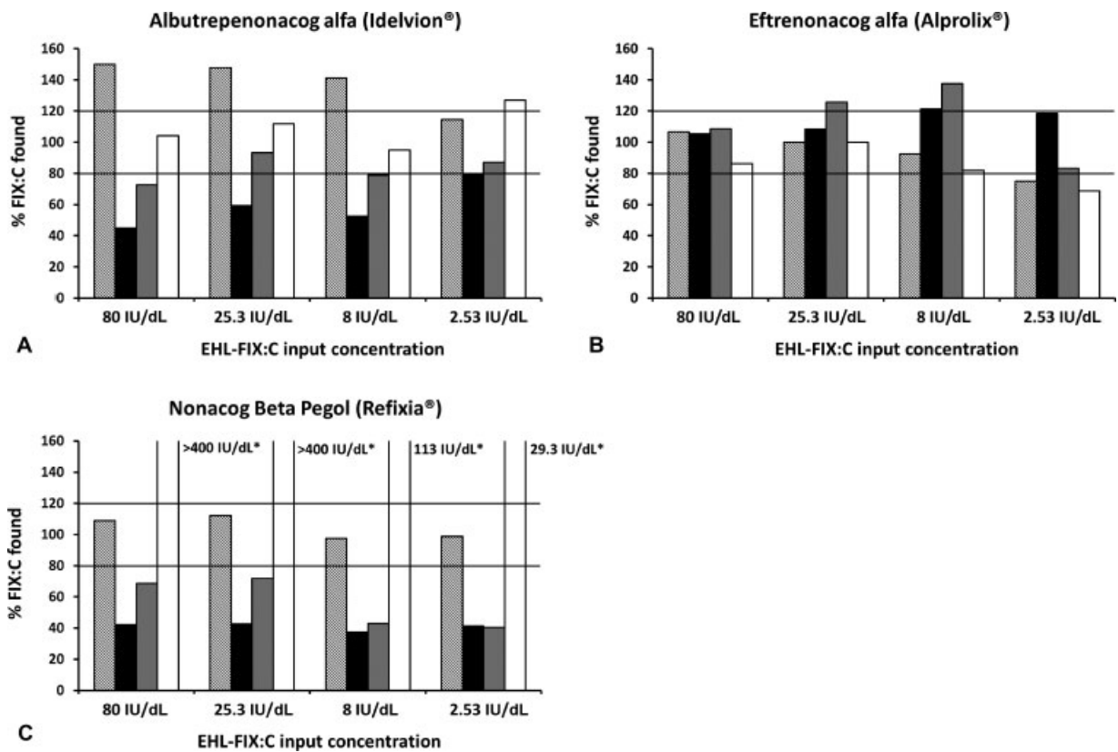
Fig. 2 Found FIX activities relative to EHL-FIX input concentrations. (A) Albutrepenocog alfa (Idelvion). (B) Eftrenonocog alfa (Alprolix). (C) Nonacog beta pegol (Refixia). *Measured absolute values. Applied test systems (from left to right)—structured columns: FIX-CSA, black columns: FIX-OSC (AFS), gray columns: FIX-OSC (AFSL), white columns: FIX-OSC (PSL). The horizontal lines represent the arbitrarily defined range of acceptance ( \pm 20\% ).
