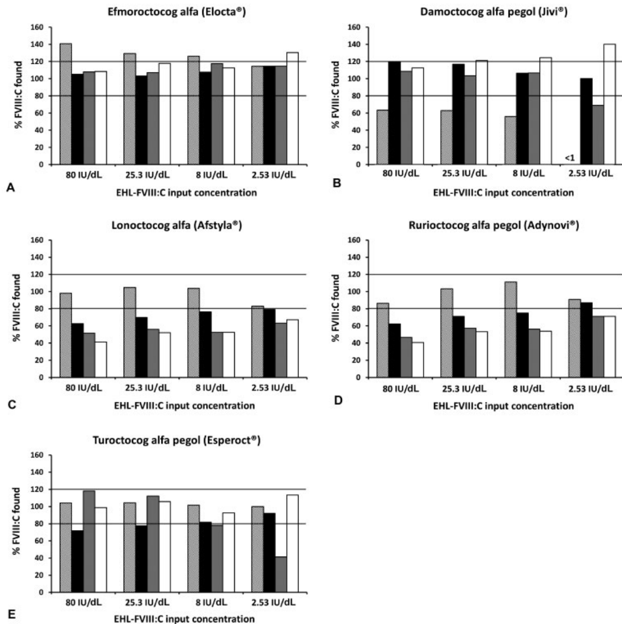
Fig. 1 Found FVIII activities relative to EHL-FVIII input concentrations. (A) Efmoroctocog alfa (Elocta). (B) Damoctocog alfa pegol (Jivi). (C) Lonooctocog alfa (Afstyla). (D) Rurioctocog alfa pegol (Adynovi). (E) Turoctocog alfa pegol (Esperoct). Applied test systems (from left to right)—structured columns: FVIII-CSA, black columns: FVIII-OSC (AFS), gray columns: FVIII-OSC (AFSL), white columns: FVIII-OSC (PSL). The horizontal lines represent the arbitrarily defined range of acceptance ( \pm 20\% ).
