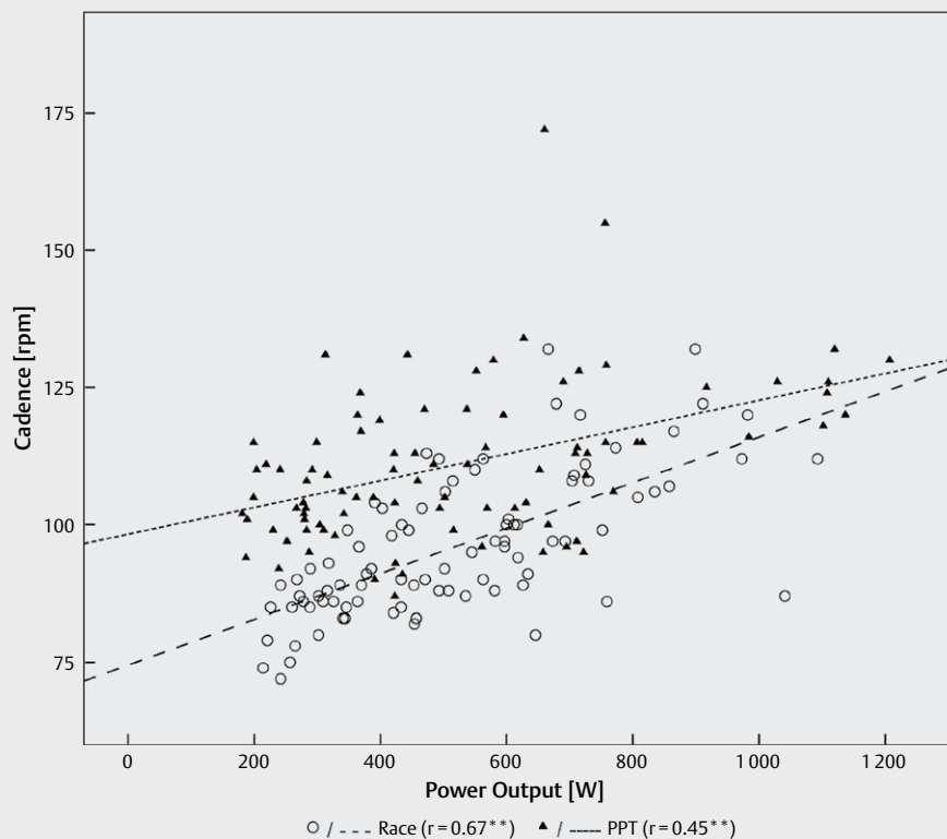
► Fig. 3 Correlation of aggregated power output and cadence; the lines represent the linear correlation for race data (Race) and the laboratory Power Profile Test (PPT); n=88 for each the Race and the PPT
