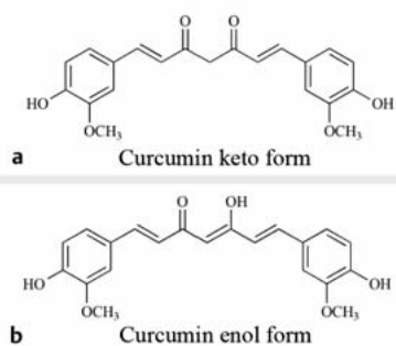
► Fig. 1 The structure of curcumin. a The structure of the curcumin keto form. b The structure of the curcumin enol form.
