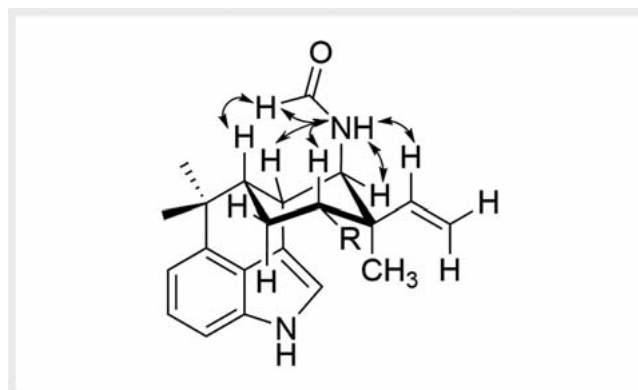
► Fig. 4 Selected NOESY correlations (arrows) of compounds 4 ( \text{R} = \text{Cl} ) and 5 ( \text{R} = \text{H} ).
