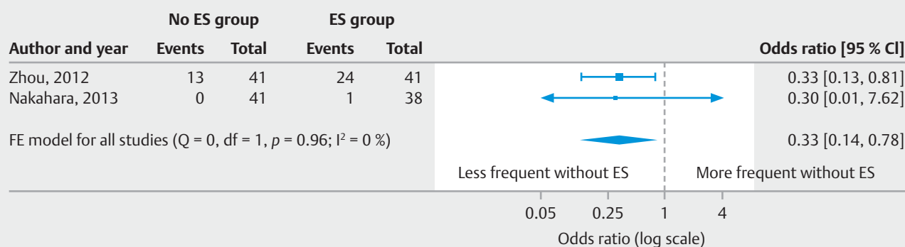
► Fig. 3 Forest plot of post-ERCP early cholangitis rates. A low between-study heterogeneity was detected ( I^2 = 0\% ; Q: 0.8 , P = 0.976 ).
