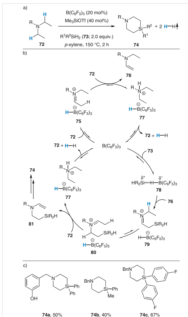
Scheme 9 Borane-mediated hydride abstraction leads to the \beta,\beta' -H silylation of tertiary amines for the synthesis of sila-piperidines
