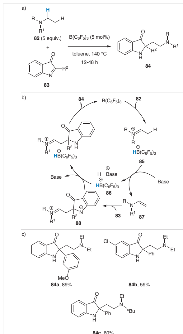
Scheme 10 Borane-mediated hydride abstraction facilitates the \beta -functionalization of amines with 3 H -indol-3-ones
